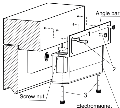
Figure 3 – Lock mounting using angle bar
