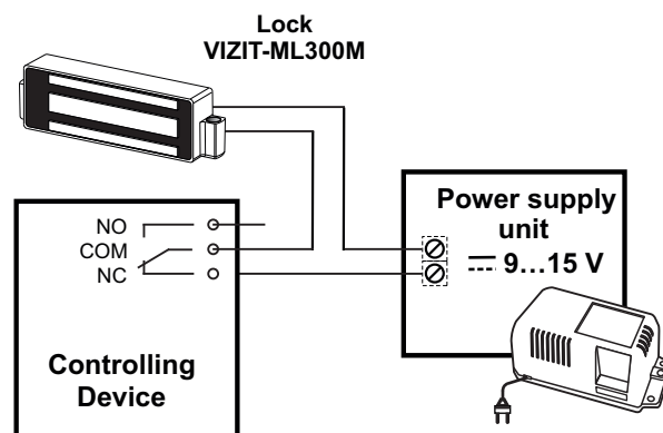
Figure 5 - Wiring diagram
