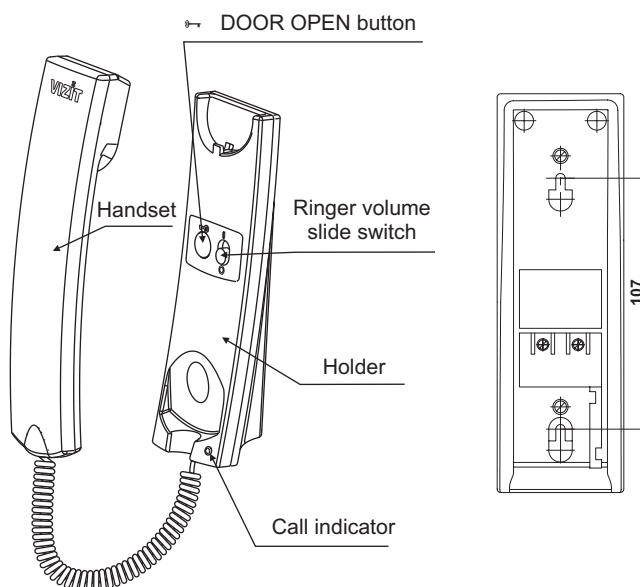
Figure 1 - Controls layout and mounting dimension
